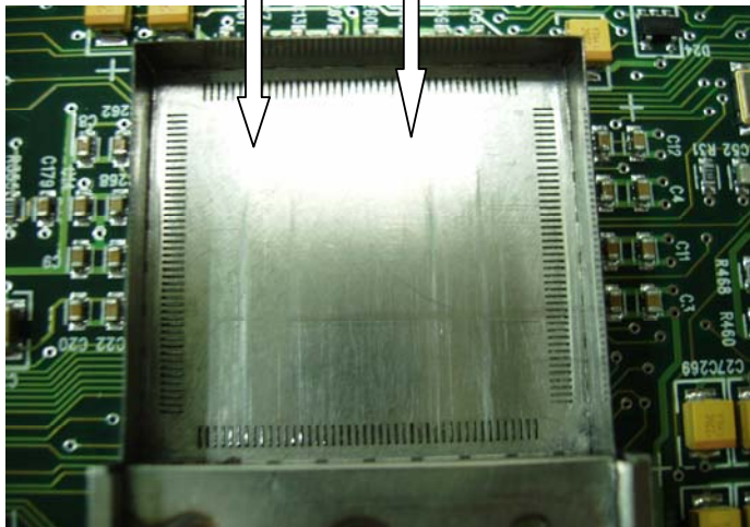
Laser cut stencil
