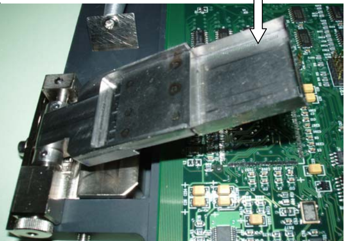
Leveled up & down mechanism with precision X & Y adjustments for accurate application of paste
