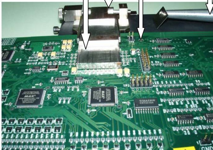
Fine pitch application of paste for mounting of components or for rework
