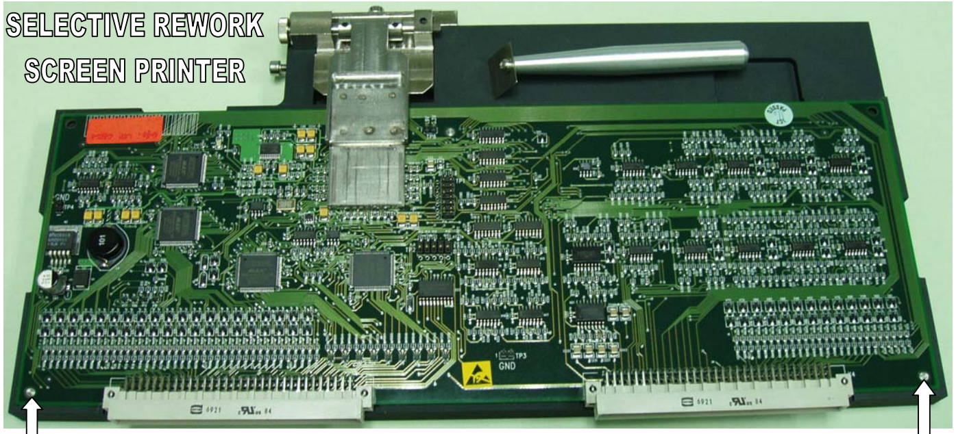
Locating pin
